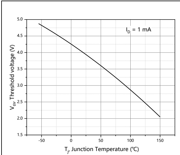
Figure 7. Threshold voltage
