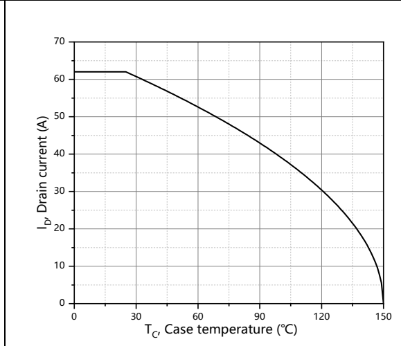
Figure 10. Drain current
