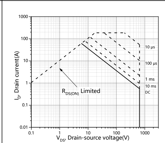
Figure 12. Safe operation area Tc=25°C
