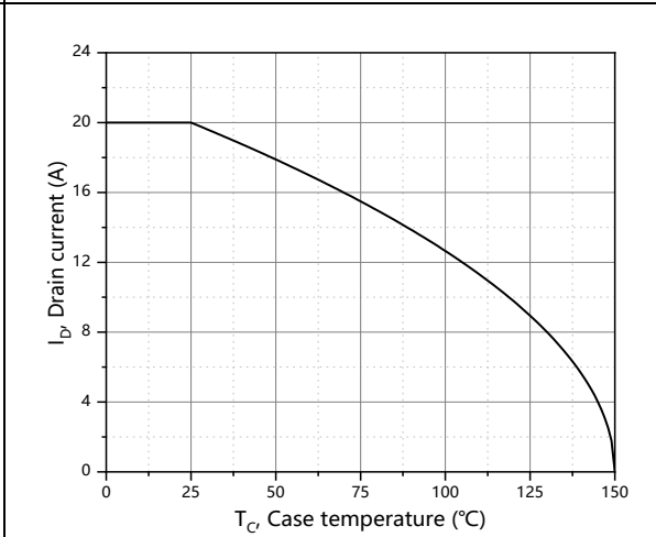
Figure 10. Drain current
