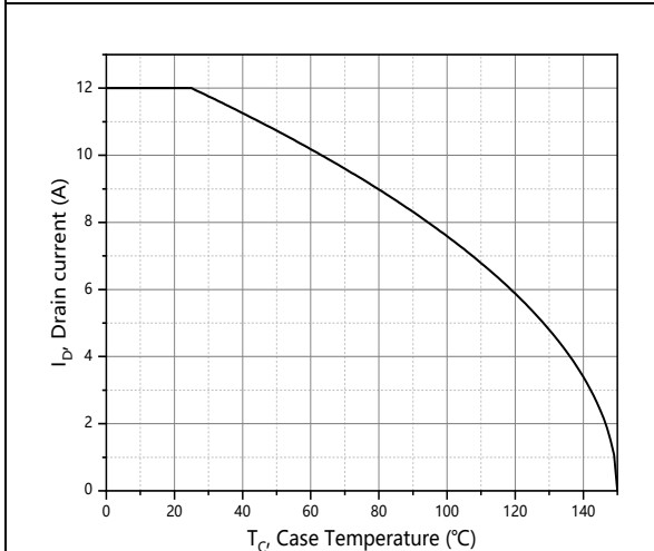
Figure 9. Drain current
