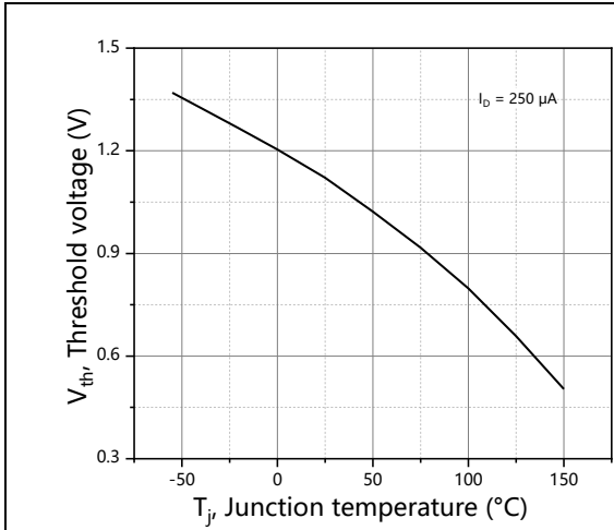
Figure 7. Threshold voltage
