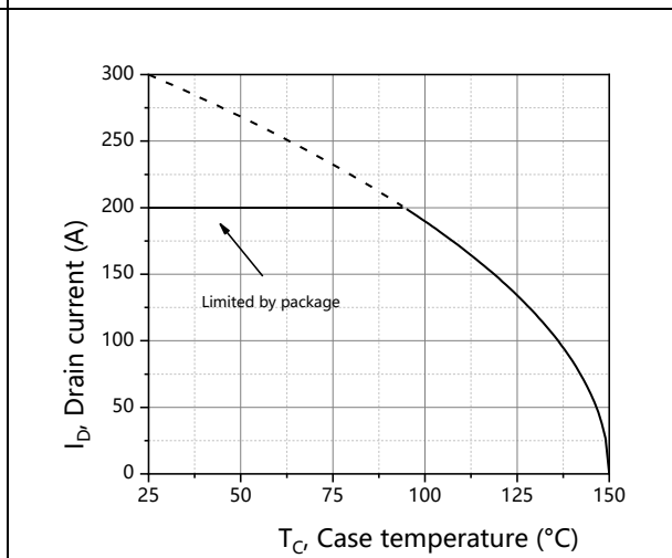
Figure 10. Drain current
