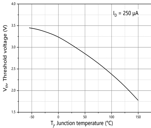
Figure 7. Threshold voltage
