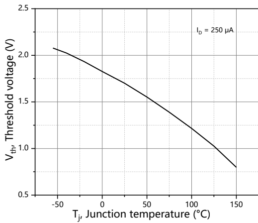
Figure 7. Threshold voltage
