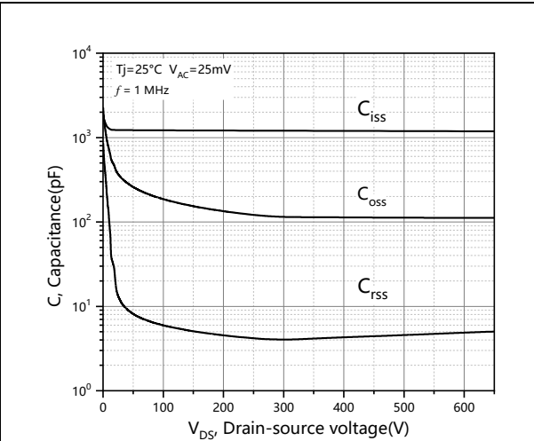
Figure 14. Capacitances vs. drain-source voltage
